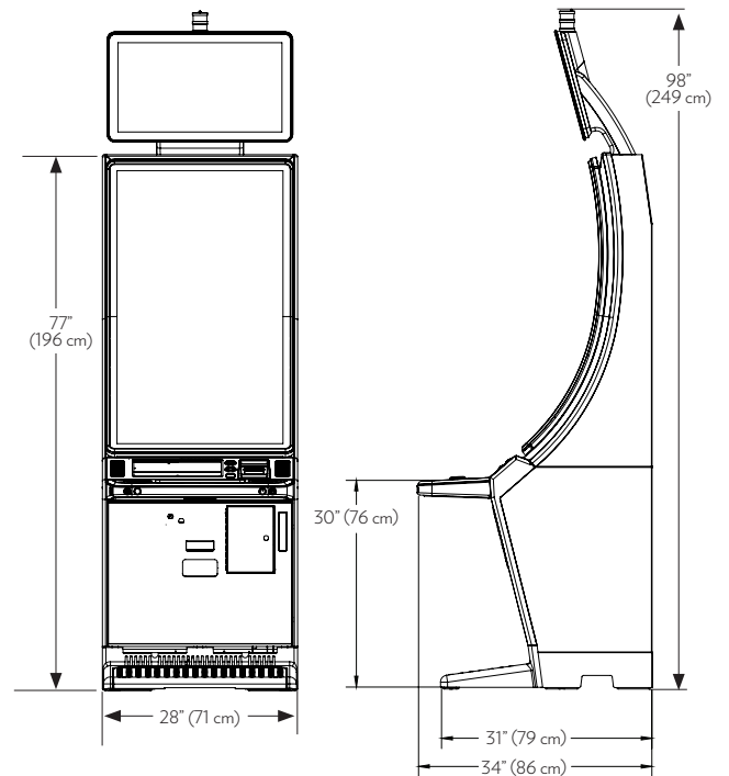
IGT PeakSlant49™ Gaming Machine Weight - 360 lbs. (163.2 kg) Projected footprint - 6.6 ft² (0.61 m²)
